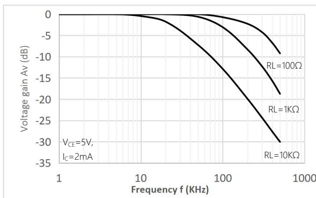
Fig.8 Frequency Response
