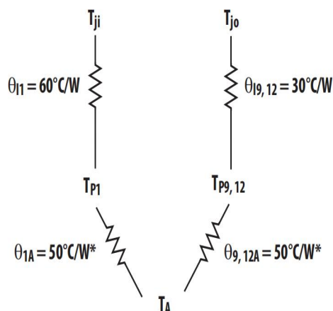
Figure. 41 HL332J thermal model
