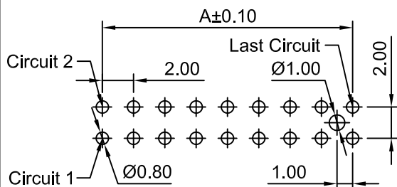
P.C.B LAYOUT TOLERANCE:±0.05
