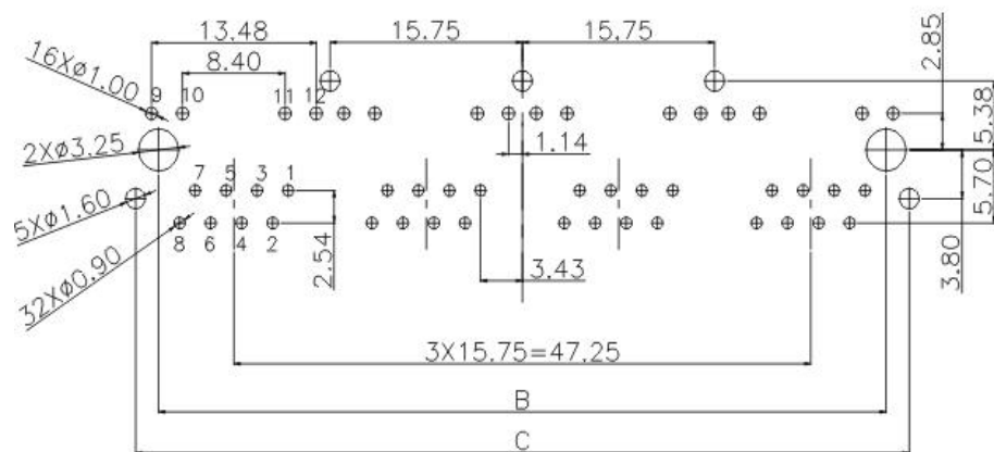
Recommended PCB Layout (PCB TOLERANCE±0.05)
