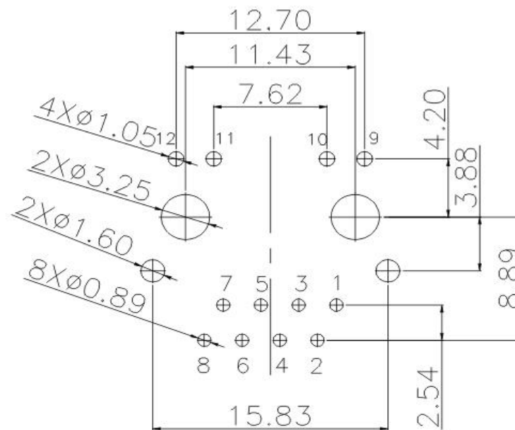
Recommended PCB Layout (PCB TOLERANCE±0.05)
