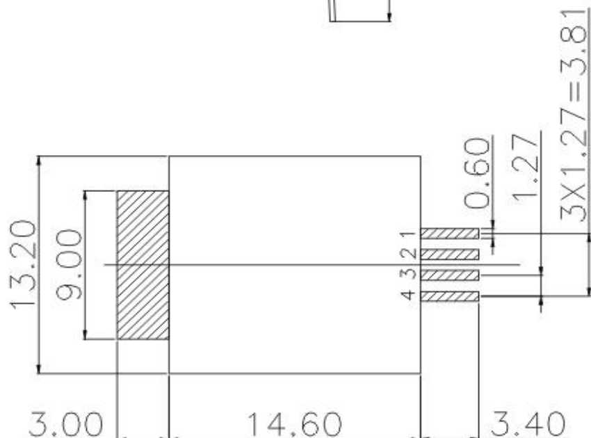
Recommended PCB Layout (PCB TOLERANCE \pm 0.05)
