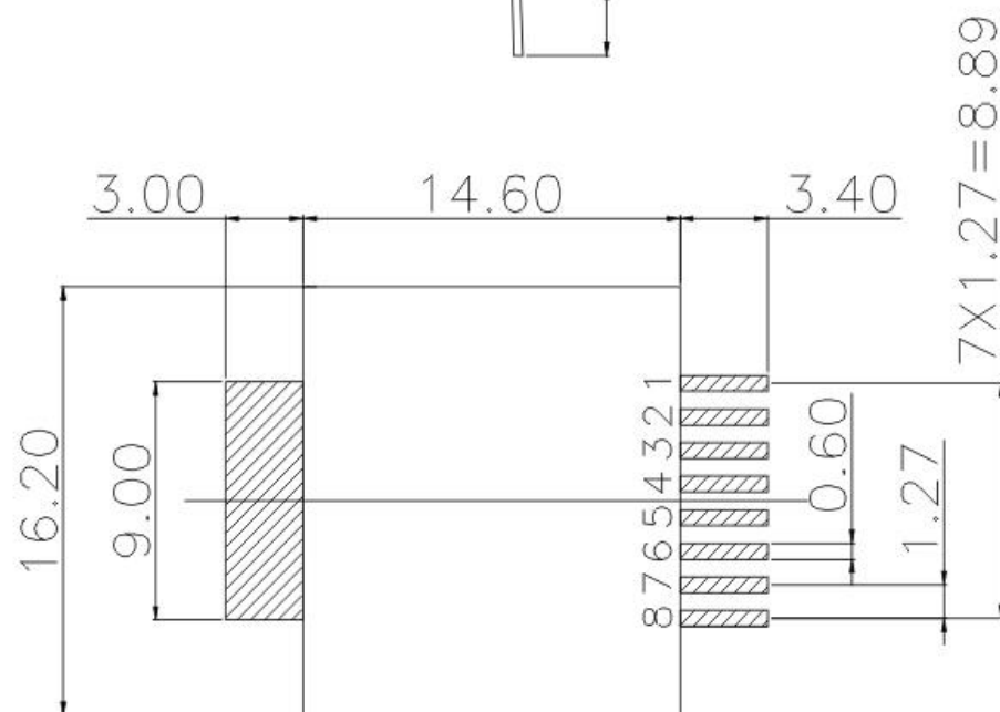
Recommended PCB Layout (PCB TOLERANCE \pm 0.05)
