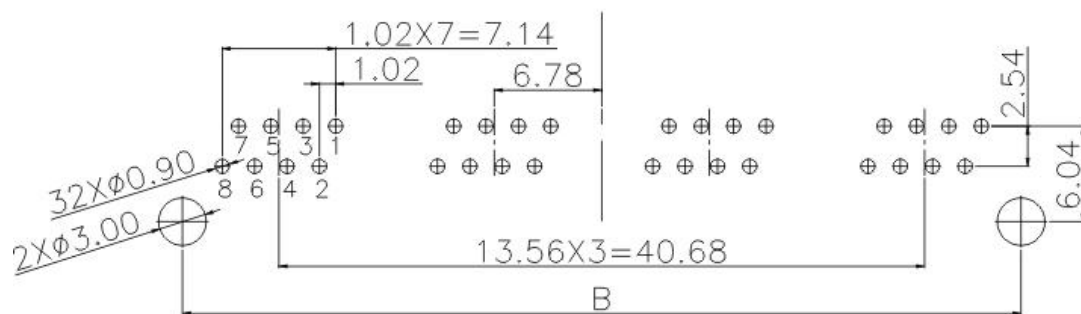
Recommended PCB Layout (PCB TOLERANCE±0.05)
