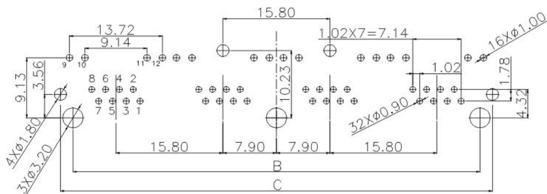
Recommended PCB Layout (PCB TOLERANCE±0.05)
