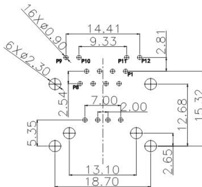
Recommended PCB Layout (PCB TOLERANCE \pm 0.05)
