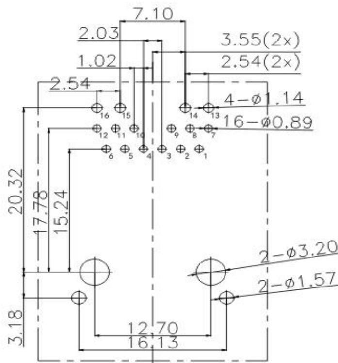
Recommended PCB Layout (PCB TOLERANCE \pm 0.05)
