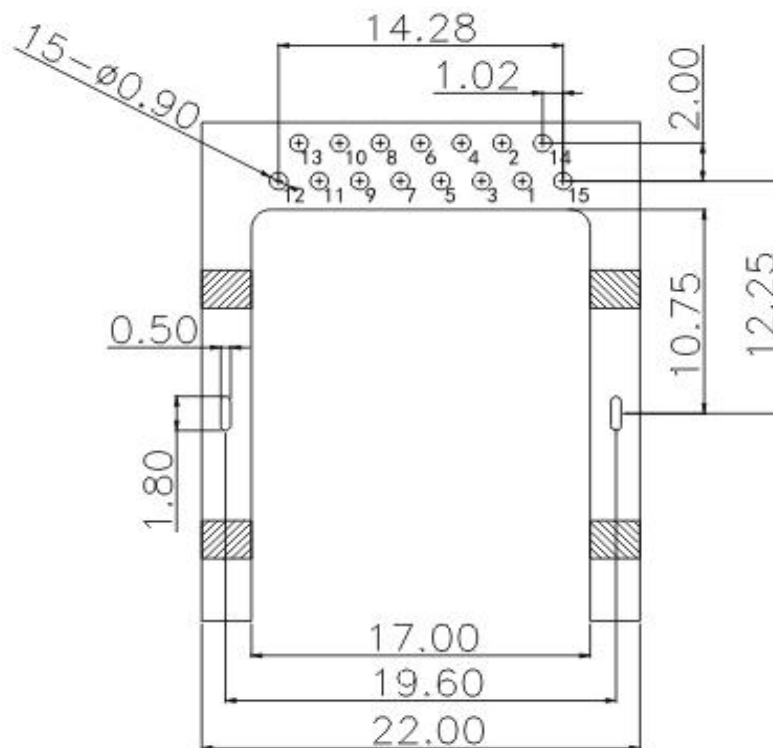
Recommended PCB Layout (PCB TOLERANCE \pm 0.05)
