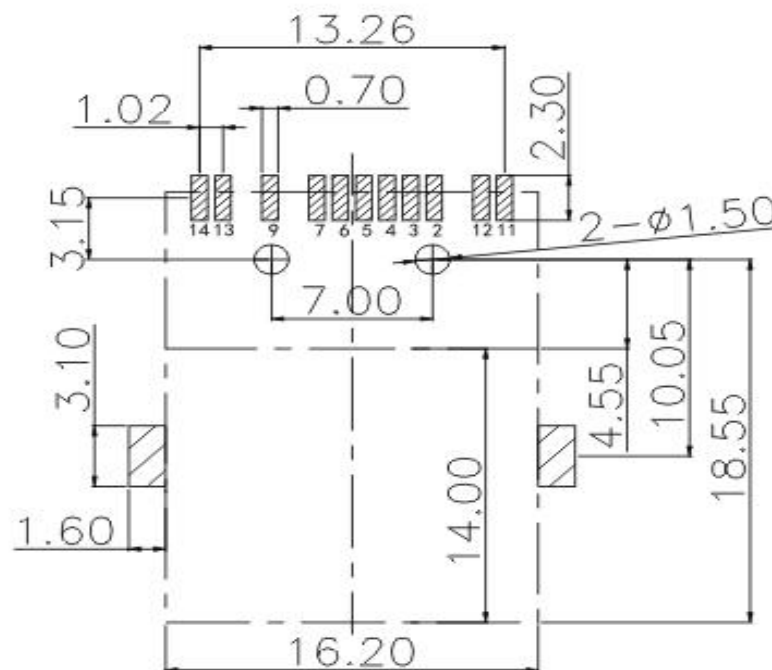
Recommended PCB Layout (PCB TOLERANCE \pm 0.05 )
