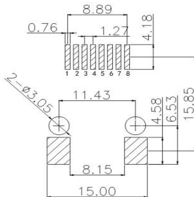
Recommended PCB Layout (PCB TOLERANCE \pm 0.05)
