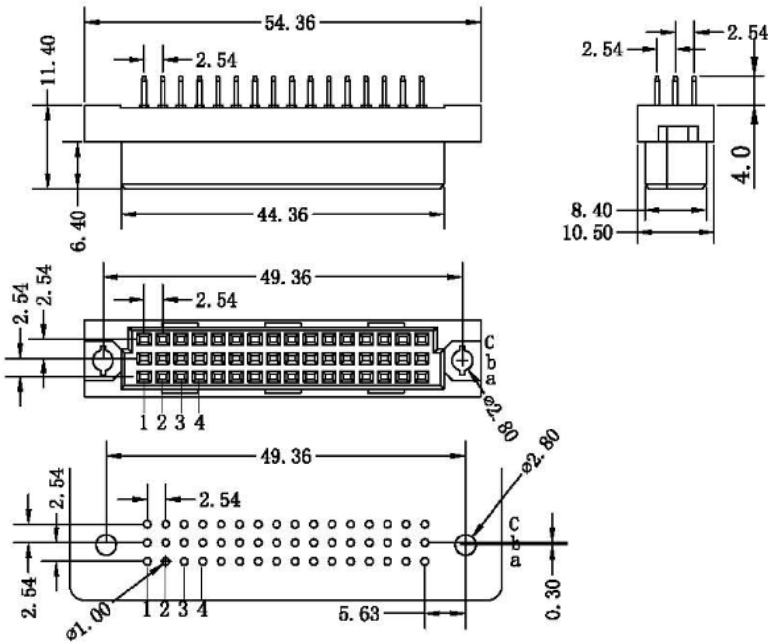
PCB LAYOUT (RECOMMENDED)
