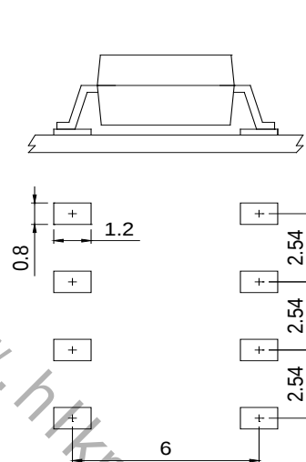
8-pin SOP
