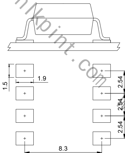
8-pin SMD
