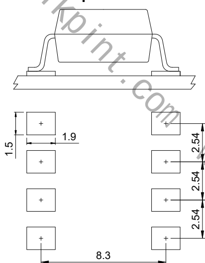
8-pin SMD
