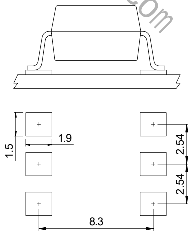
6-pin SMD
