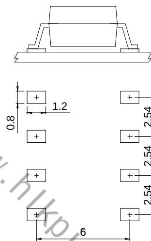
8-pin SOP
