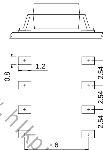
8-pin SOP
