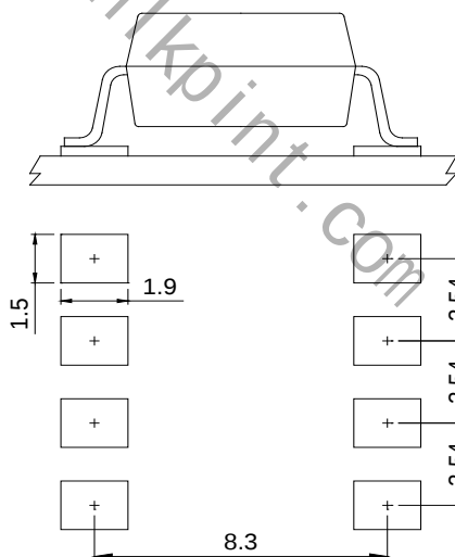
8-pin SMD
